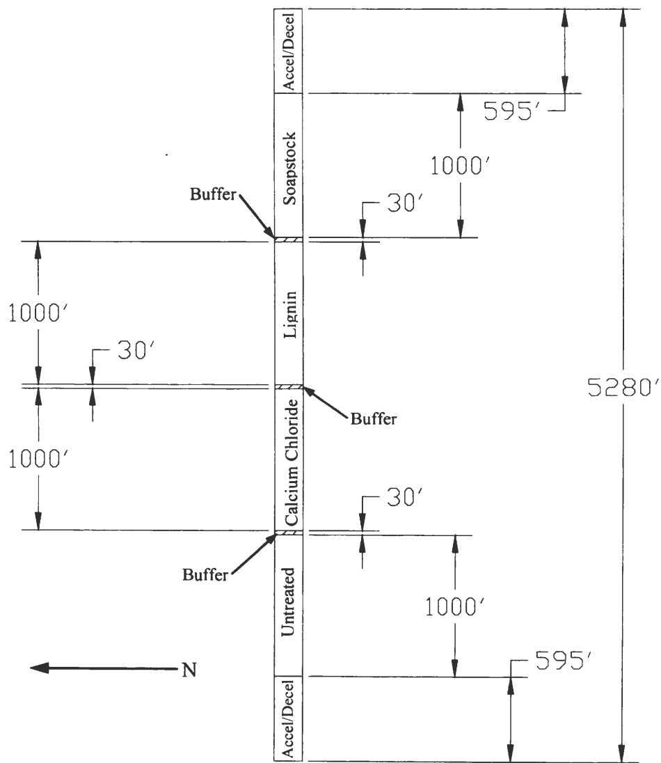
Figure 3.4.2. Zumwalt Road test section plan.
