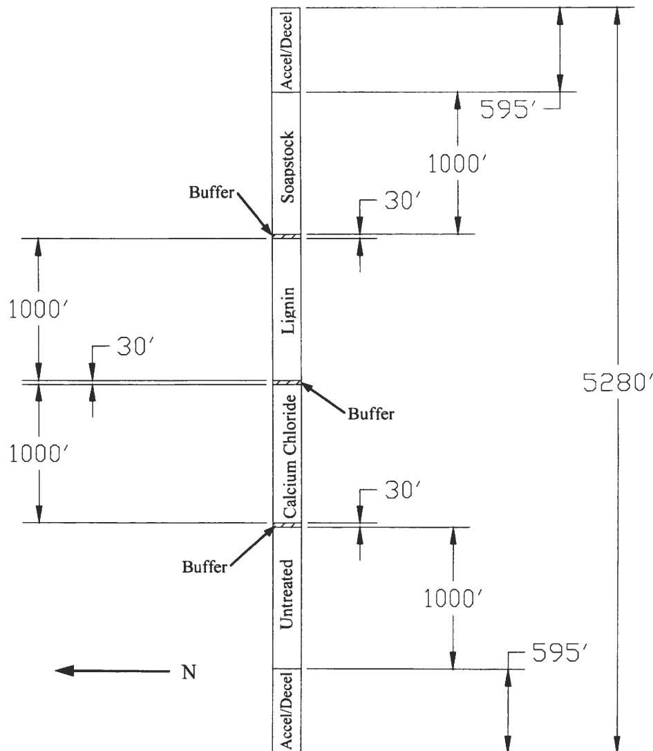
Figure 3.4.1. 260 th Street test section plan.
