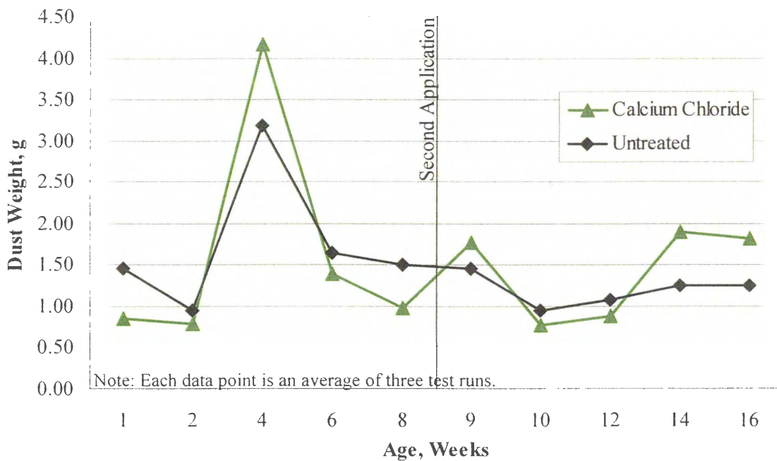
Figure 6.1.11. Grant Avenue 16 week calcium chloride dust measurement results.
