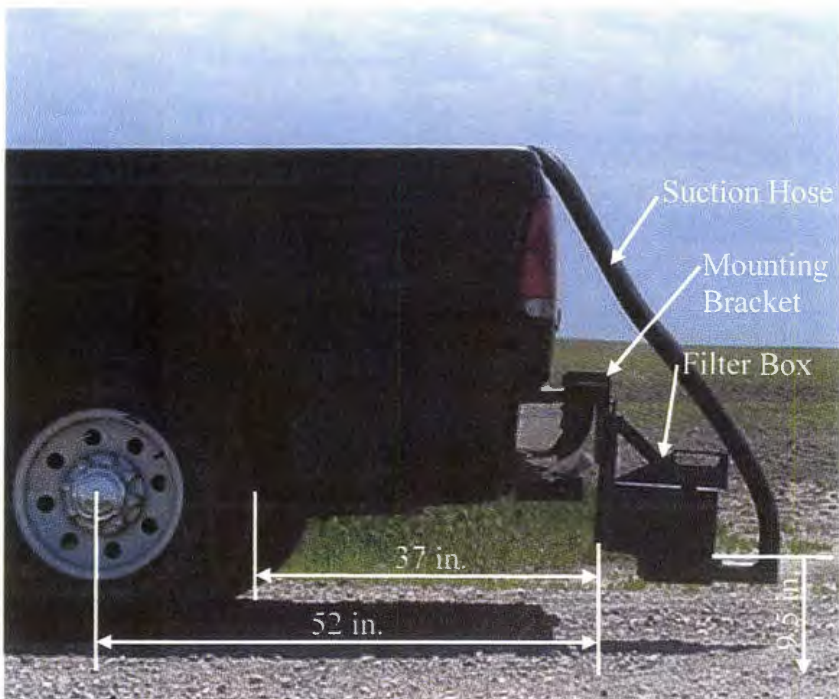
Figure 5.1.4. Mounted dustometer dimensions.
