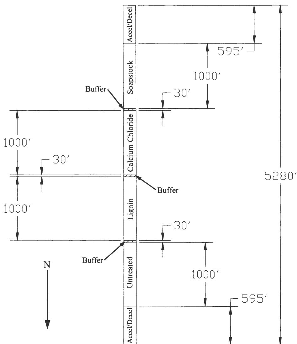
Figure 3.4.3. Grant Avenue test section plan.
