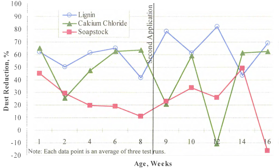
Figure 6.2.3. South 530 th Avenue 16 week dust reduction results.
