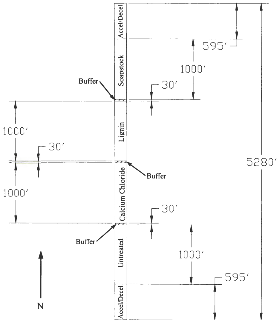
Figure 3.4.4. South 530 th Avenue test section plan.
